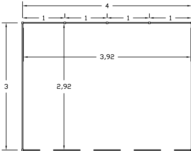
FLOOR PLANT
